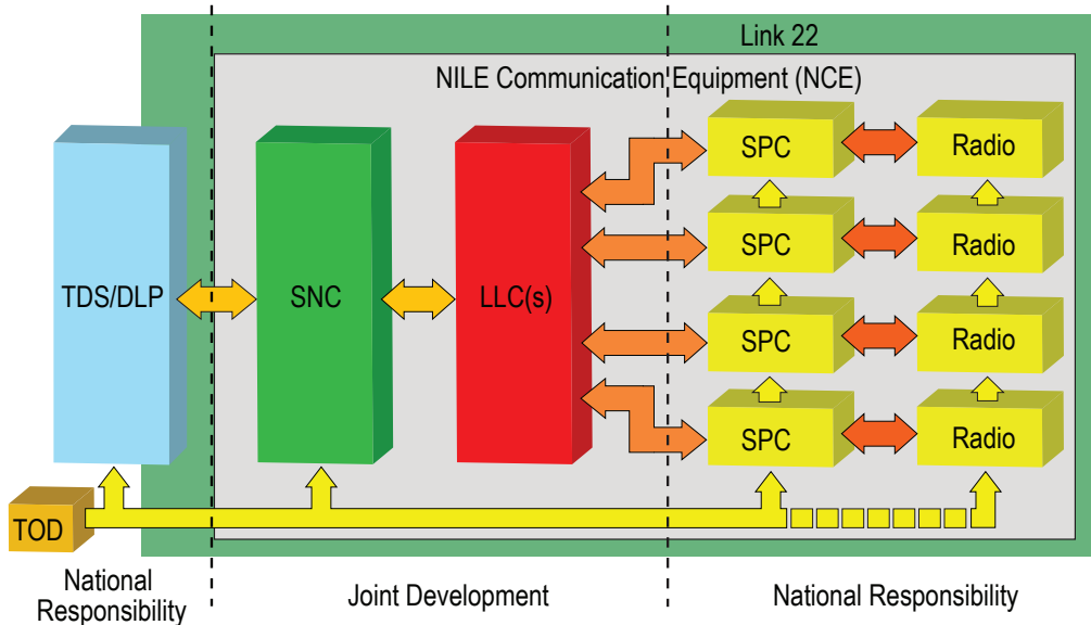
Figure 4-11. Link 22 System Architecture.
